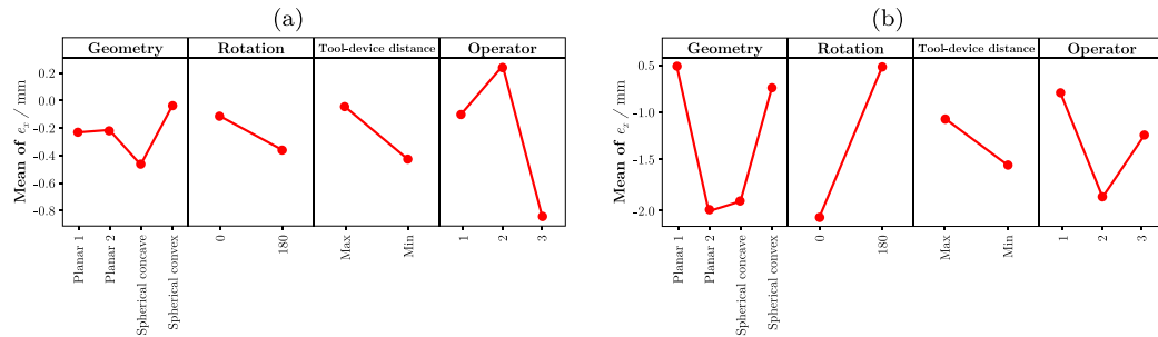
Fig. 12. Main effect plots for e_x due to (a) HoloLens 2 and (b) Intel RealSense.
