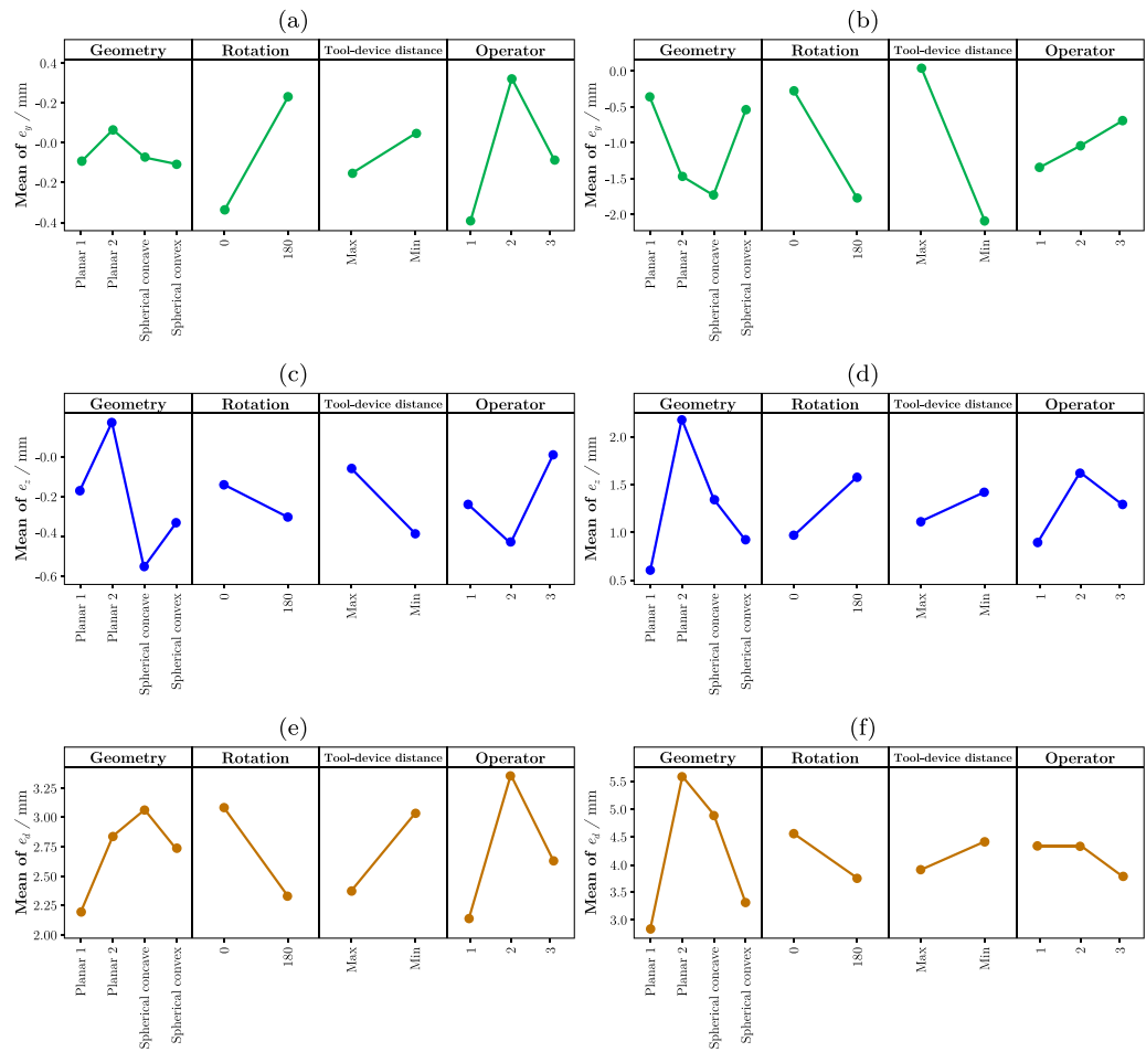
Fig. A.15. Main effect plots for: (a) e_y due to HoloLens 2, (b) e_y due to RealSense, (c) e_z due to HoloLens 2, (d) e_z due to RealSense, (e) e_d due to HoloLens 2, and (f) e_d due to RealSense.
