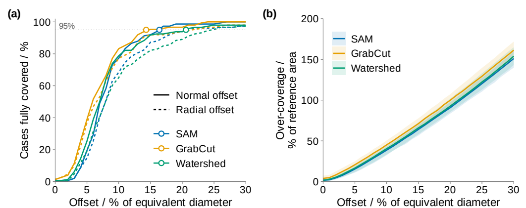
Figure 12. Perilesional offset (all valid cases; n = 149 , 149 and 146 for SAM, GrabCut and watershed). (a) Percentage of cases in which the patch enlarged by a given offset covers the reference entirely, for the normal offset of Equation (15) (solid lines) and for the radial offset of Algorithm 1 (dashed lines); the offset is expressed as a percentage of the equivalent diameter of the reference; circles mark \delta^*(0.95) and the dotted line the 95% level. (b) Cost of the margin: median over-coverage produced by a normal offset, as a percentage of the reference area (band: interquartile range).
