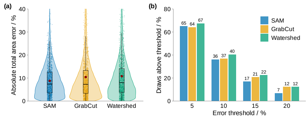
Figure 9. Monte Carlo distribution of the absolute total area error |\varepsilon_{\text{patch}}| (all valid cases; 20,000 draws per back-end): (a) distribution per back-end (violin and box computed on all draws; box: median and interquartile range; red dot: mean; dots: 1200 of the draws; 1.7% of the draws lie above the displayed 40%); (b) percentage of draws exceeding thresholds of 5%, 10%, 15% and 20%. Each draw combines a resampled clinical segmentation error with a simulated scale error and a printing error (Equation (12)); the figure therefore shows a propagated estimate, not measured clinical cases.
