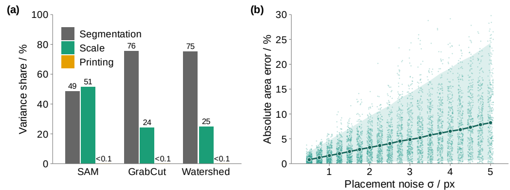
Figure 8. (a) Share of the variance of the total area error \varepsilon_{\text{patch}} contributed by the segmentation, scale and printing terms, E_k^2/E_{\text{patch}}^2 (Equation (14)), per back-end (all valid cases; n = 149, 149 and 146 for SAM, GrabCut and watershed). (b) Simulated scale term: absolute relative area error against the placement noise \sigma of the two calibration points, for a reference of L = 117 px (line: median and band: 5th to 95th percentile of 20,000 draws; dots: 300 of the draws for each value of \sigma , those above 30% not being displayed). The budget of Table 5 uses \sigma = 3 px.
